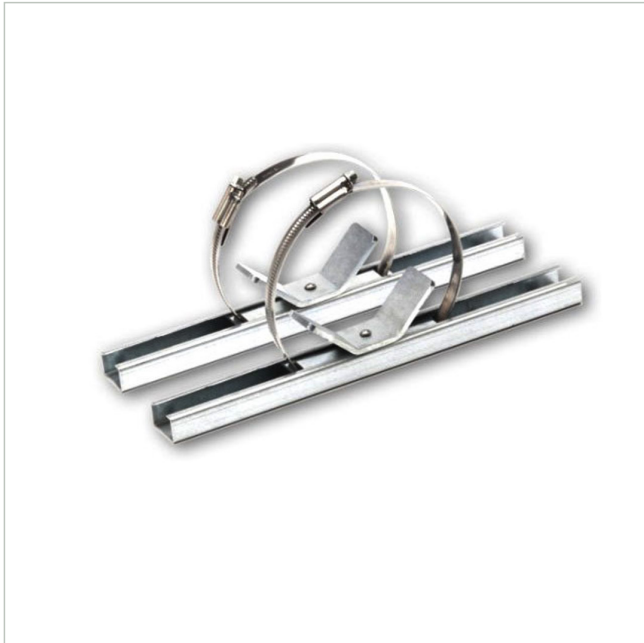
Pole mounting for CUS-WST and SOL-IQbox series set (2pcs)
