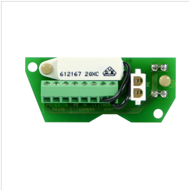
Cable Connection Board w. Thermostat and Fuse for VHM Housing, "EC" Series
